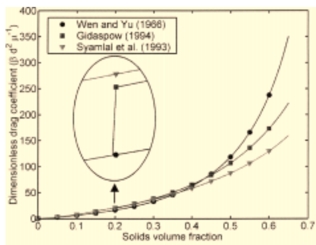
Figure 6. Different expressions for the interphase drag coefficient as a function of solid volume-fraction: Re_p = 45 .
