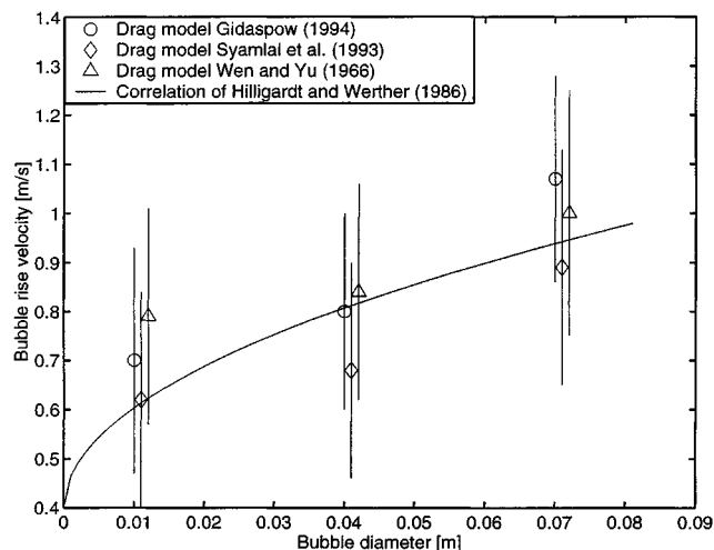
Figure 13. Predicted bubble rise velocity as a function of the bubble diameter at U = 0.54 m/s based on different drag models and compared to the experimental correlation of Hilligardt and Werther (1986).
