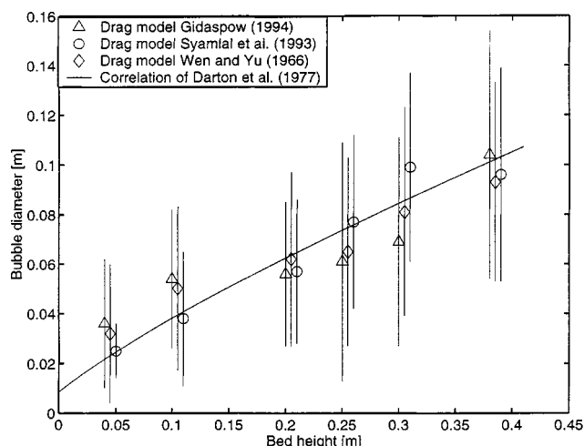
Figure 12. Predicted bubble size as a function of bed height at U = 0.54 m/s based on different drag models and compared to the correlation of Darton et al. (1977).
