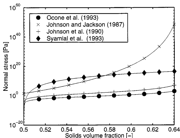
Figure 5. Different expressions for the frictional normal stress.
