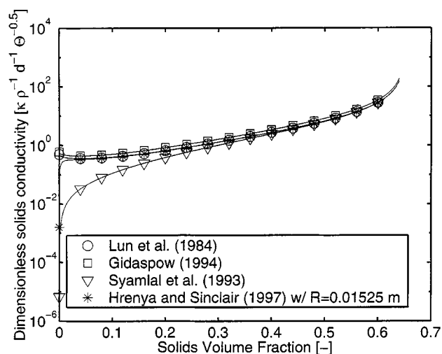
Figure 2. Comparison of solids thermal conductivity from different kinetic theory models: e = 0.9 , \epsilon_{\max} = 0.65 .
